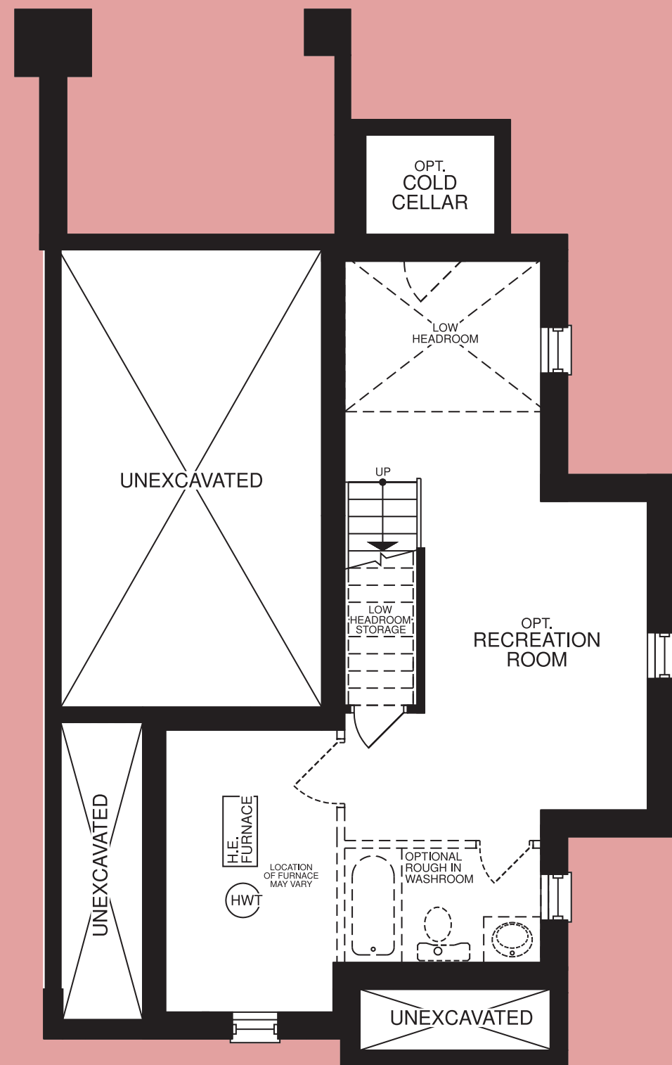
BASEMENT PLAN ELEVATION A
