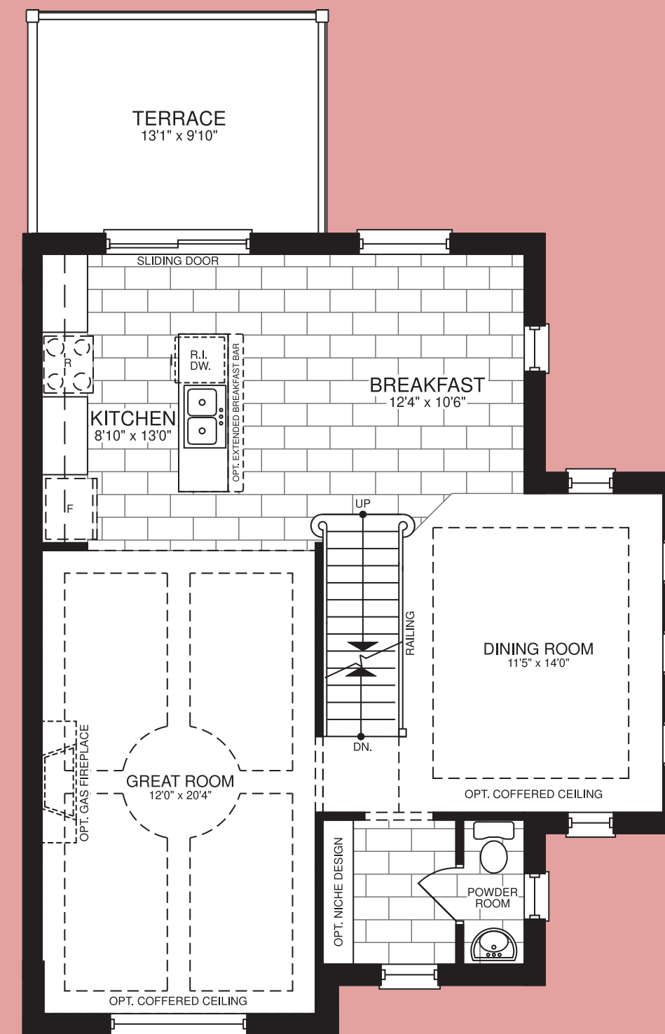
SECOND FLOOR PLAN ELEVATION A
